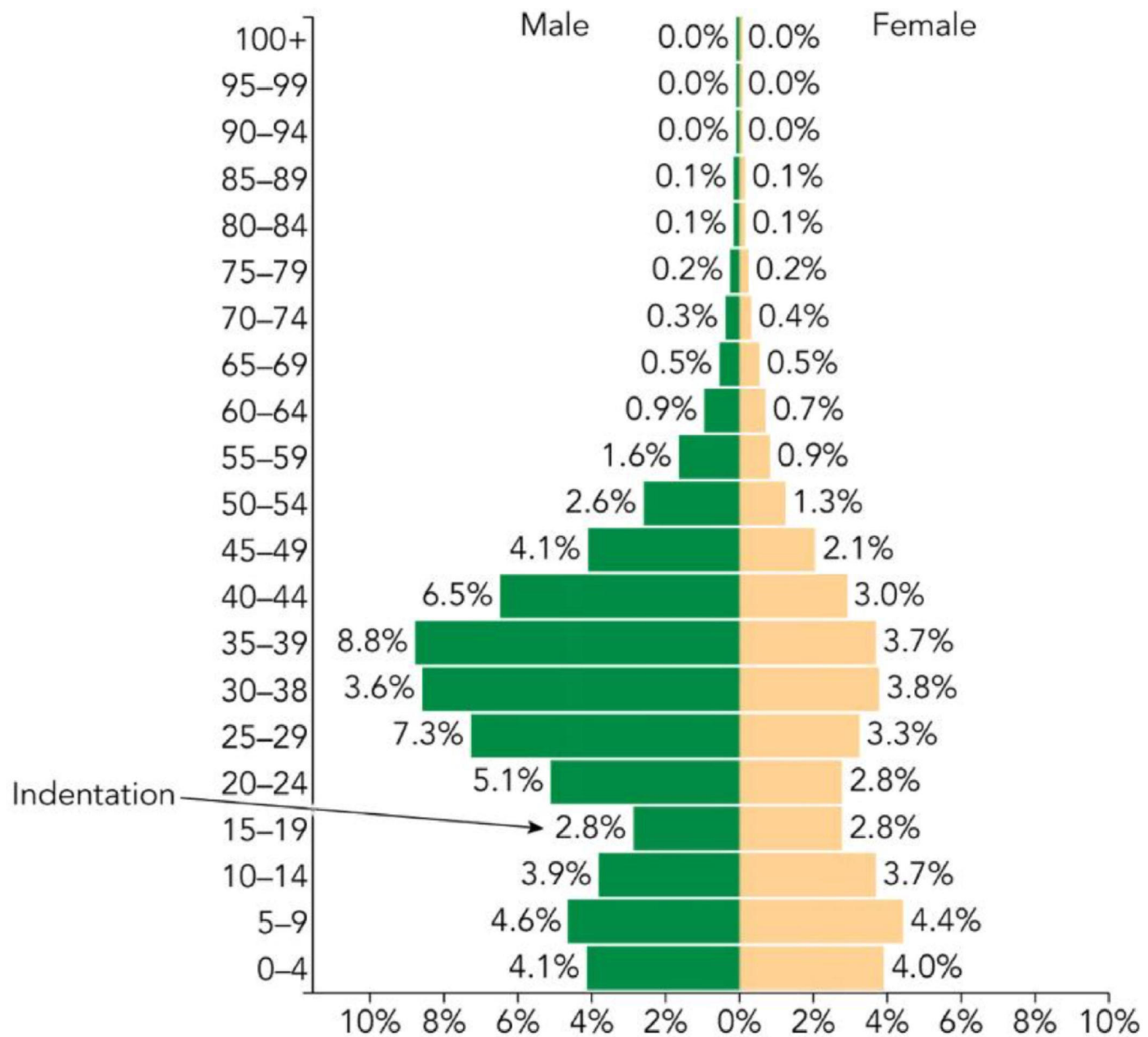
Figure 6.1: A population pyramid showing 'indentations'
